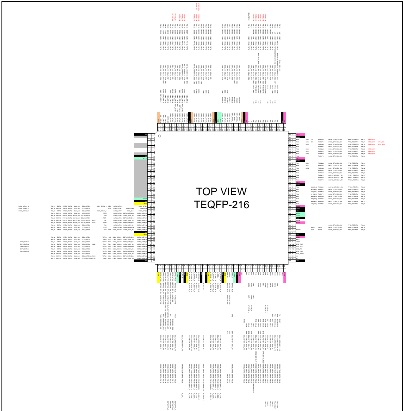
Figure 4-7: TEQFP-216 (S6J323CLxx)
