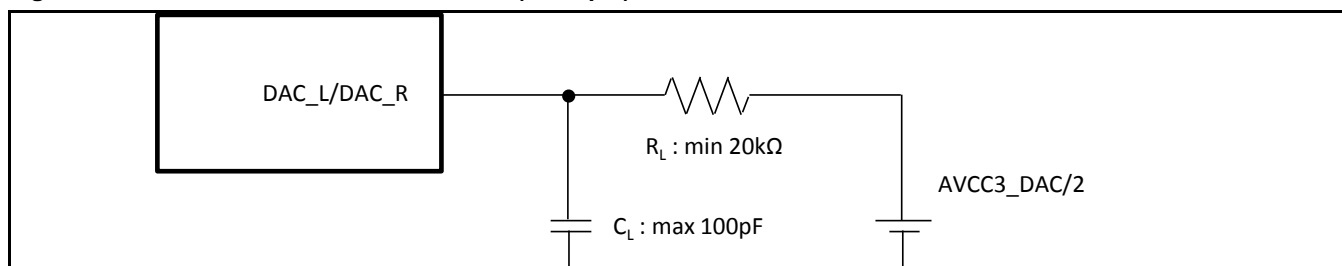
Figure 8-9: R_L is Connected to AVCC_DAC/2 (Example)
